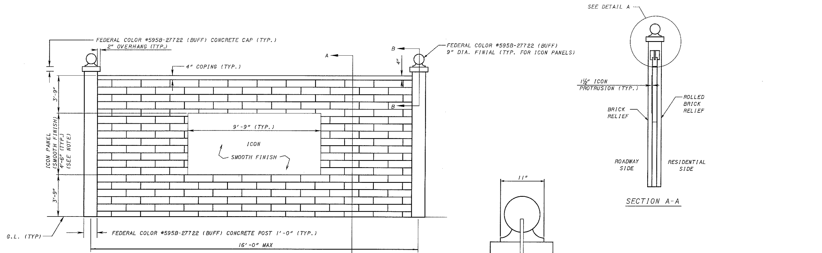
NOISE BARRIER ELEVATION (HIGHWAY SIDE)
